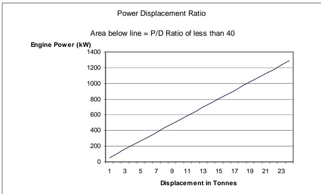
Chart for Power Displacement Ratio:
